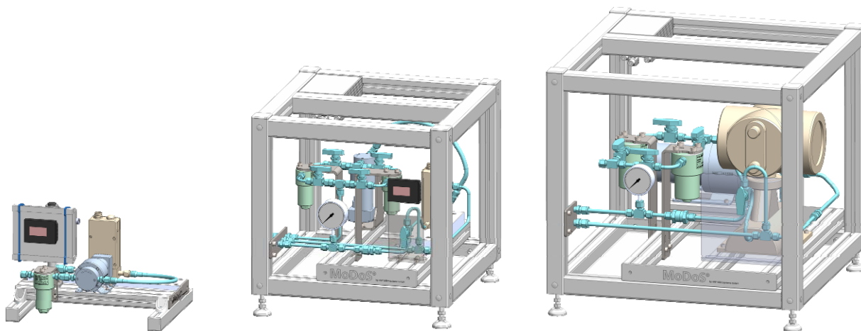
Closed loop controlled volume flow
